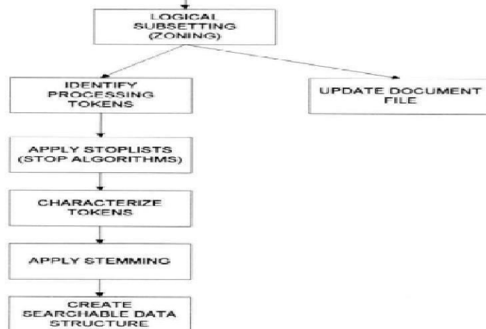
Figure 1.5 The Text Normalization Process
