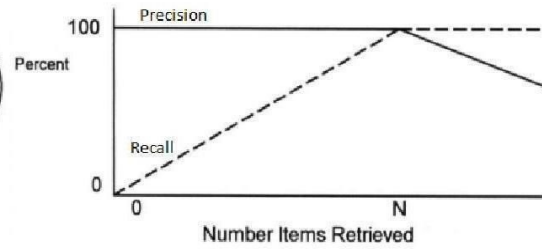
1.2a Ideal Precision and Recall
