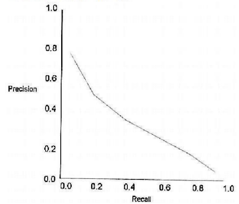
Figure 1.2c Achievable Precision/Recall Graph
