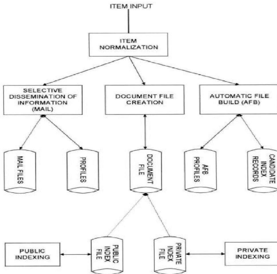
Figure 1.4 Total Information Retrieval System
