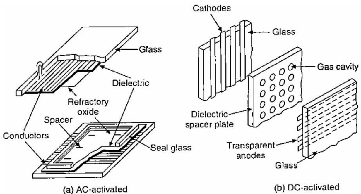
Basic structure of gas discharge plasma displays.
