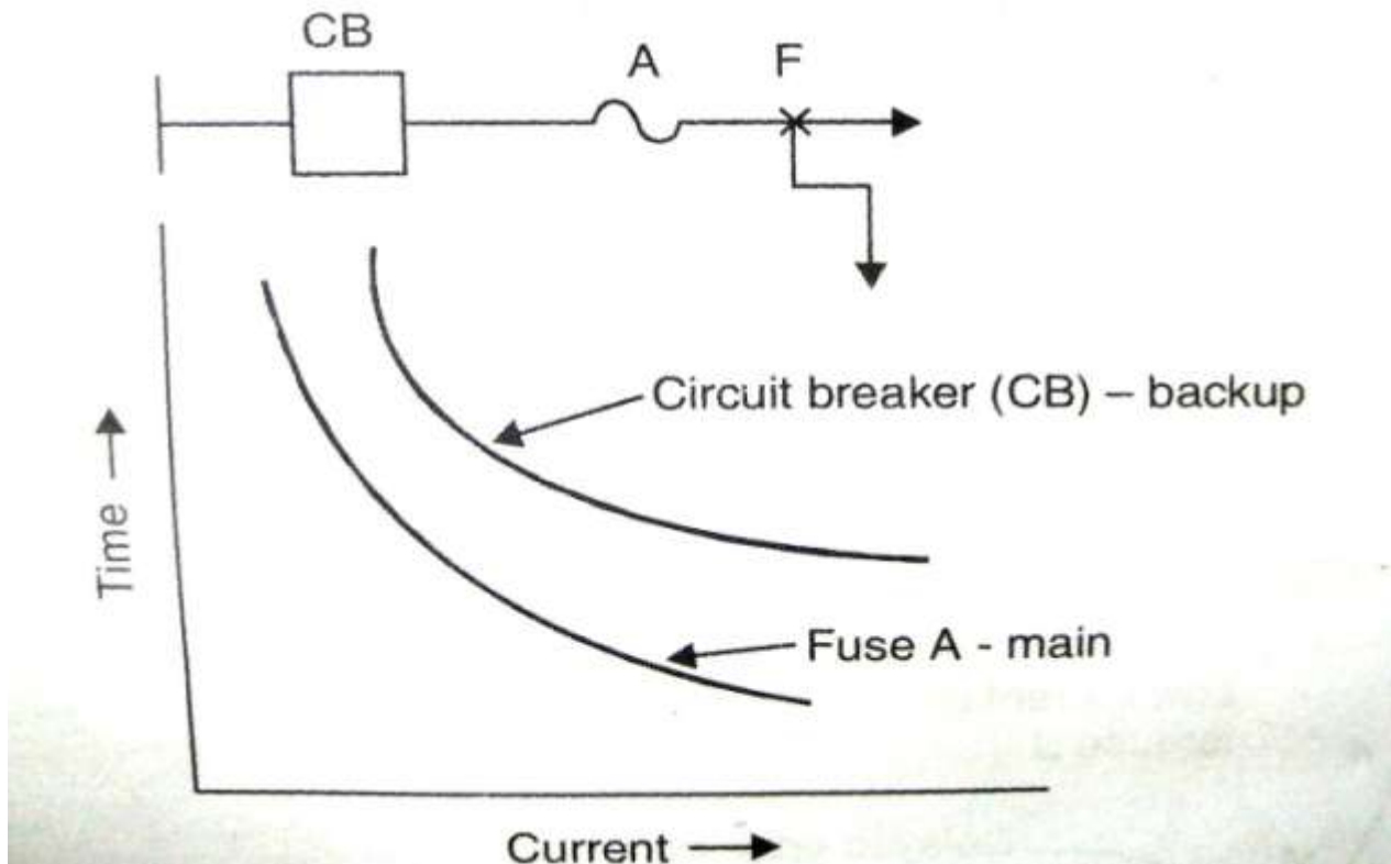
FIG FUSE GIVES MAIN PROTECTION AND CIRCUIT BREAKER GIVEN BACK UP
