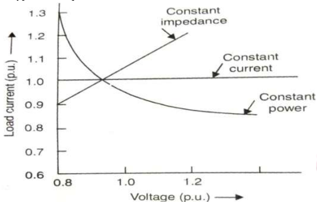
FIG RELATION BETWEEN LOAD CURRENT AND NODE VOLTAGE FOR SIMPLE LOAD TYPES
