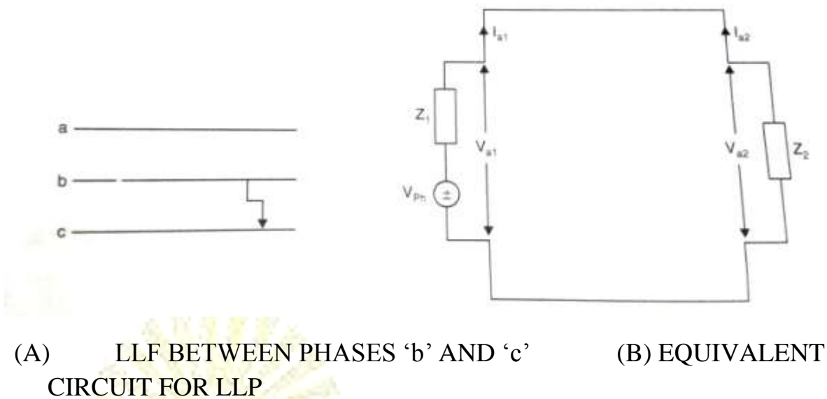
FIG LINE TO LINE FAULT
