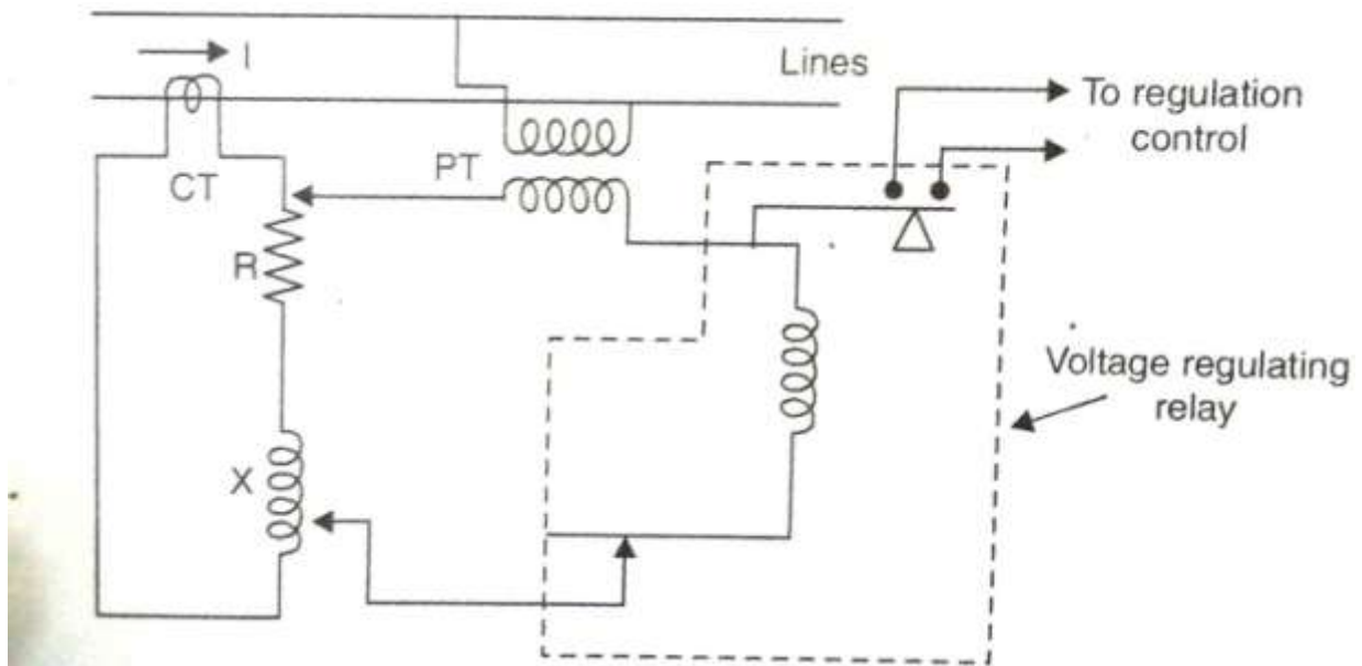
FIG 6.6 SCHEMATIC DIAGRAM OF LINE DROP COMPENSATOR
