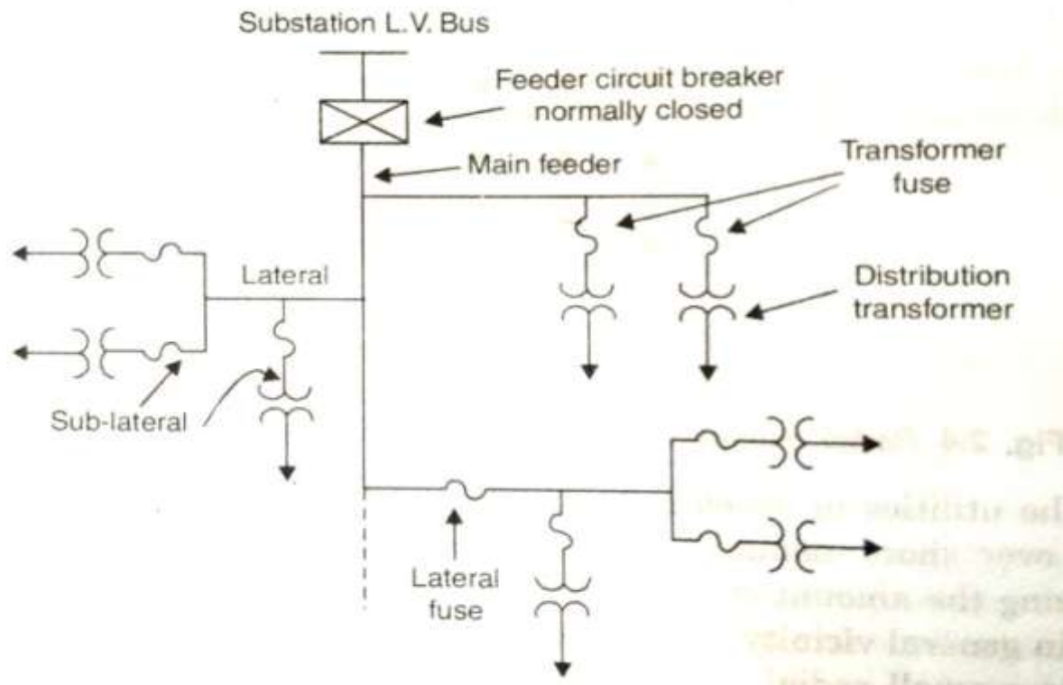
FIG 2.2 BASIC RADIAL PRIMARY FEEDER CONFIGURATION
