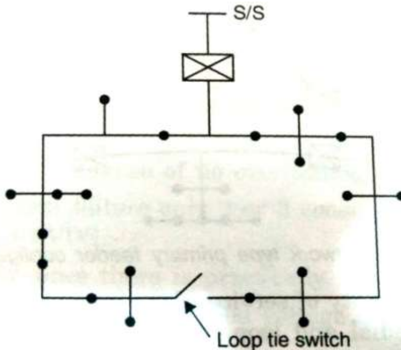
FIG 2.5 LOOP PRIMARY FEEDER CONFIGURATION
