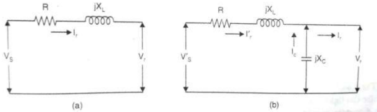
FIG 5.3 SINGLE LINE DIAGRAM WITHOUT AND WITH SHUNT COMPENSATION
