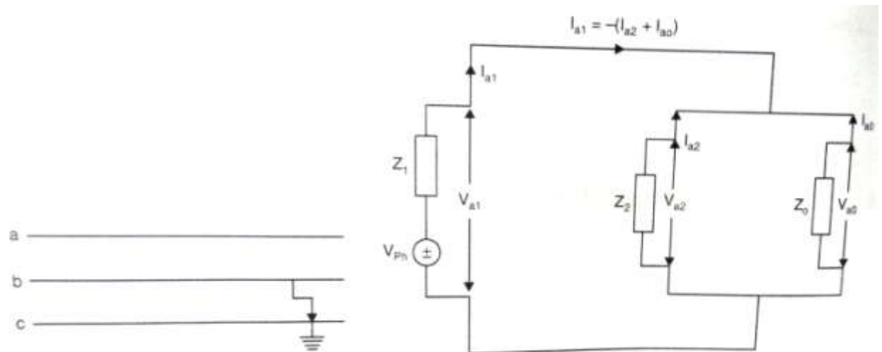
(A) DLGF IN BETWEEN PHASE 'b' AND 'c' (B) EQUIVALENT CIRCUIT FOR DLGF
