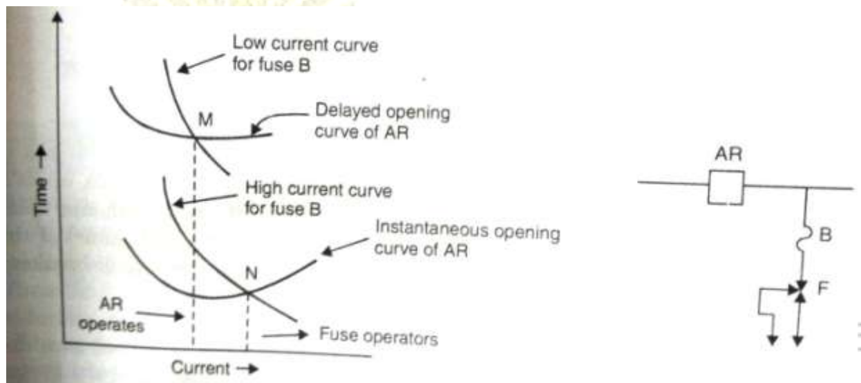
FIG AUTO-RECLOSER AND FUSE CO-ORDINATION
