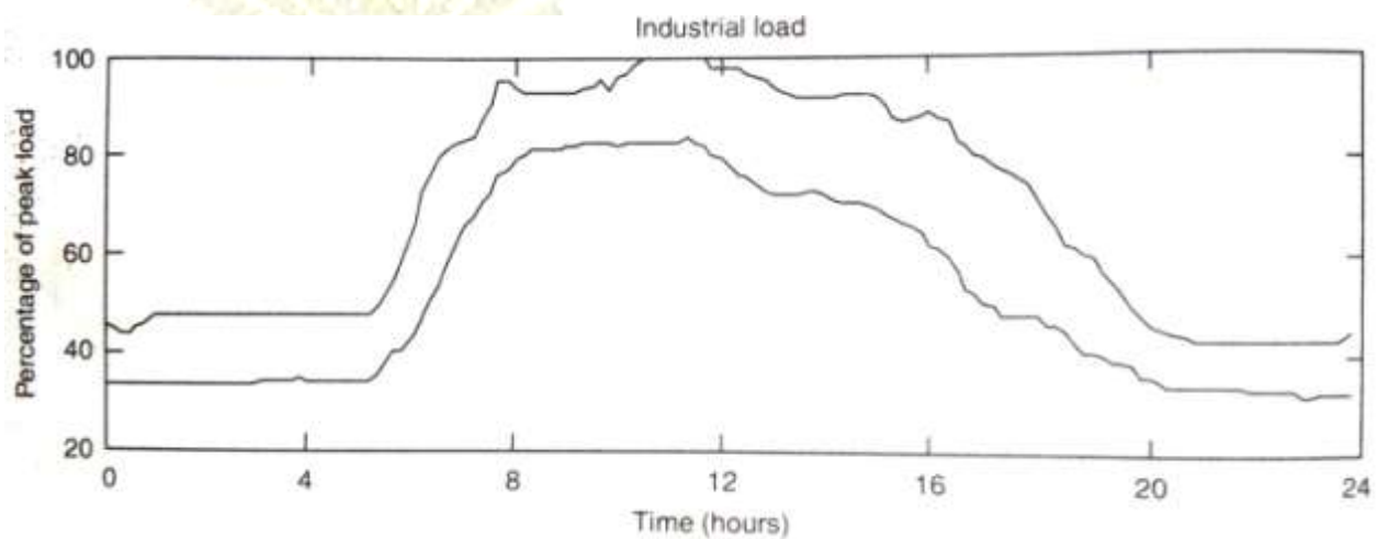
FIG Industrial load curve in percentage of peak load
