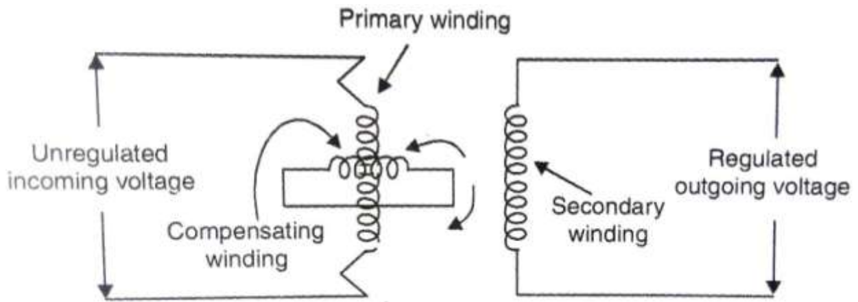
FIG 6.4 INDUCTION TYPE OF VOLTAGE REGULATOR
