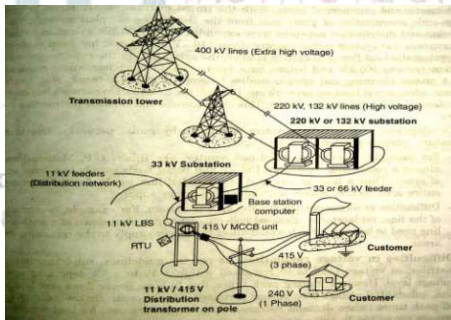
T&D System Consists of Several Levels of Power Delivery Equipment
