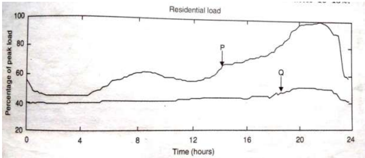
FIG Residential load curve in percentage of peak load
