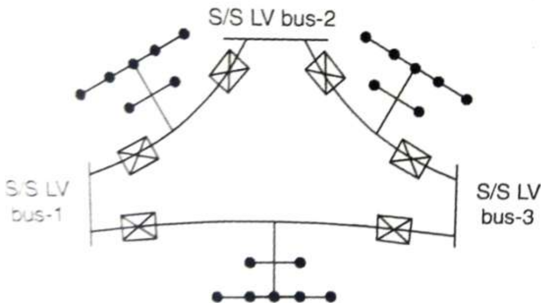
FIG 2.6 NETWORK TYPE PRIMARY FEEDER CONFIGURATION
