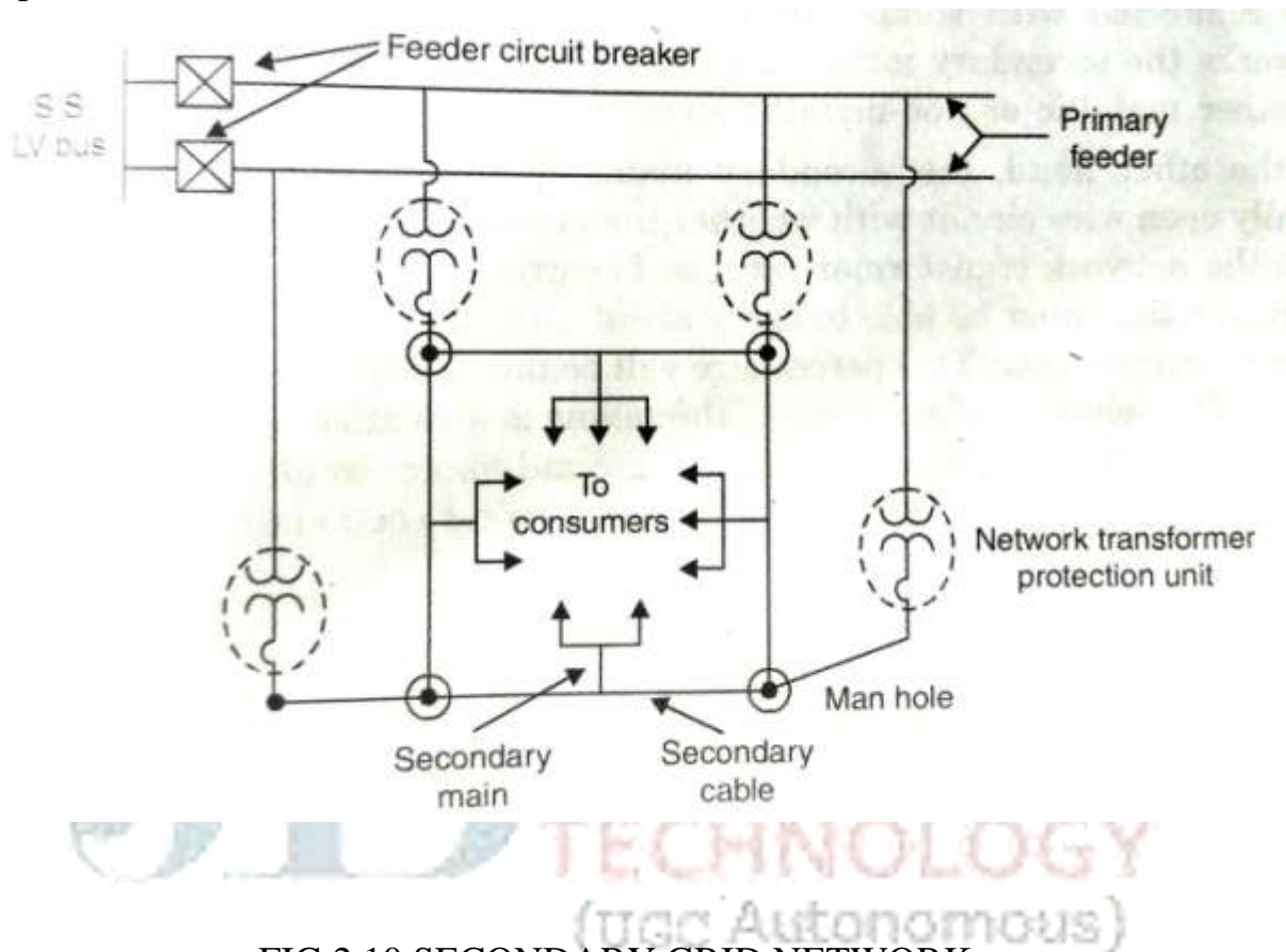
FIG 2.10 SECONDARY GRID NETWORK
