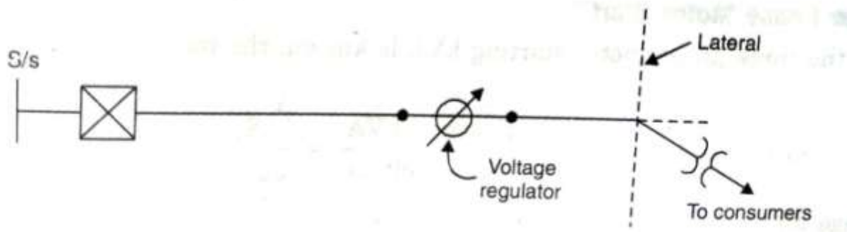
FIG 6.7 LOCATION OF FEEDER VOLTAGE REGULATOR
