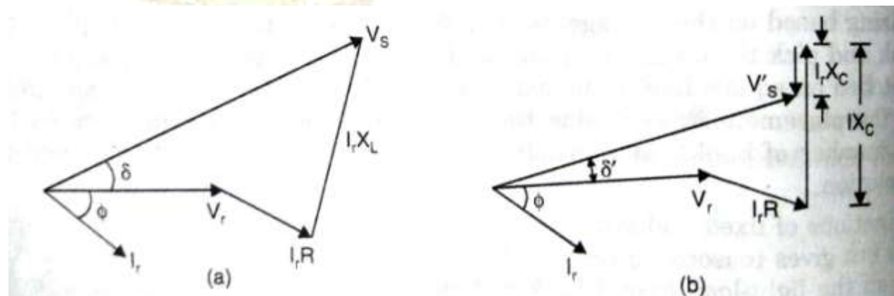
FIG 6.2 PHASOR DIAGRAM OF FIG 6.1(a) AND (B) RESPECTIVELY
