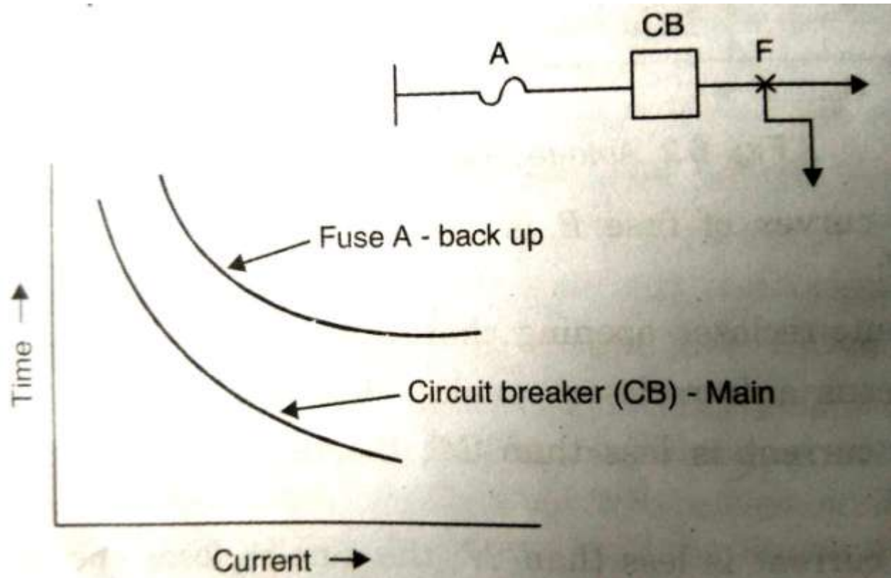
FIG CIRCUIT BREAKER GIVES MAIN PROTECTION AND FUSE GIVEN BACK UP
