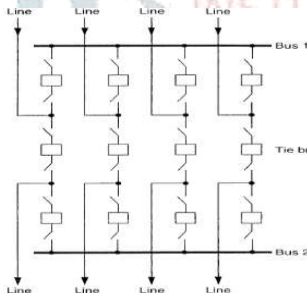
A typical breaker-and-a-half scheme.
