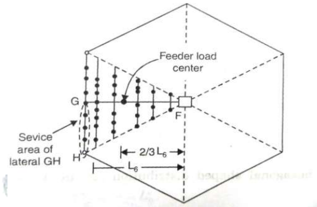
FIG HEXAGONAL SHAPED SERVICE AREA OF DISTRIBUTION SUBSTATION
