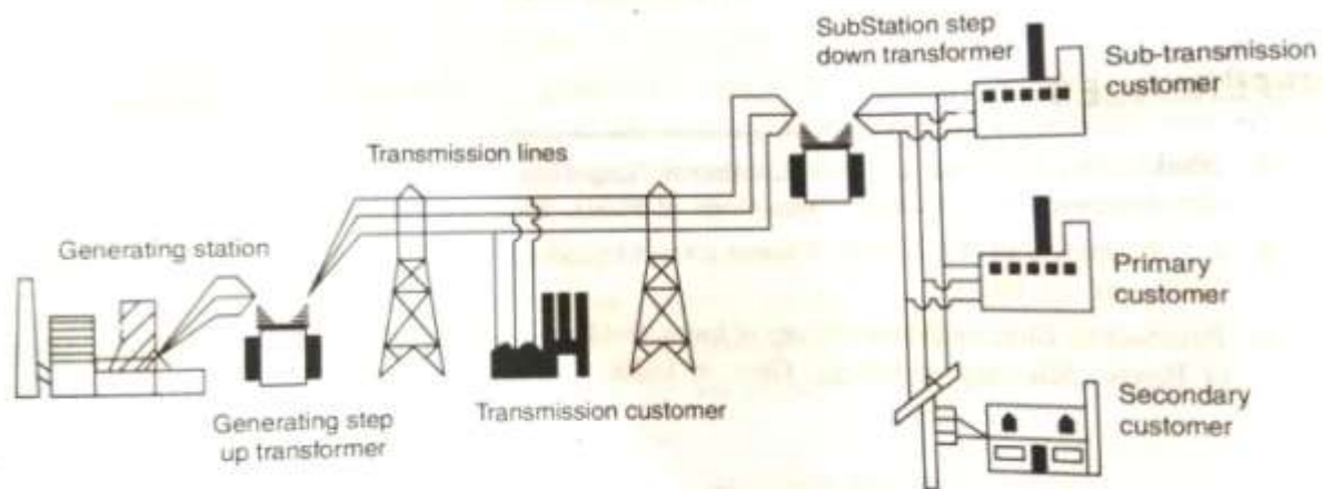
FIG 2.1 Schematic diagram of power system
