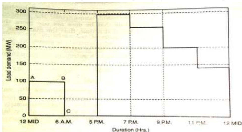
FIG Daily load curve of domestic consumer
