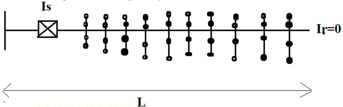
Fig 2 uniformly distributed load of the circuit
