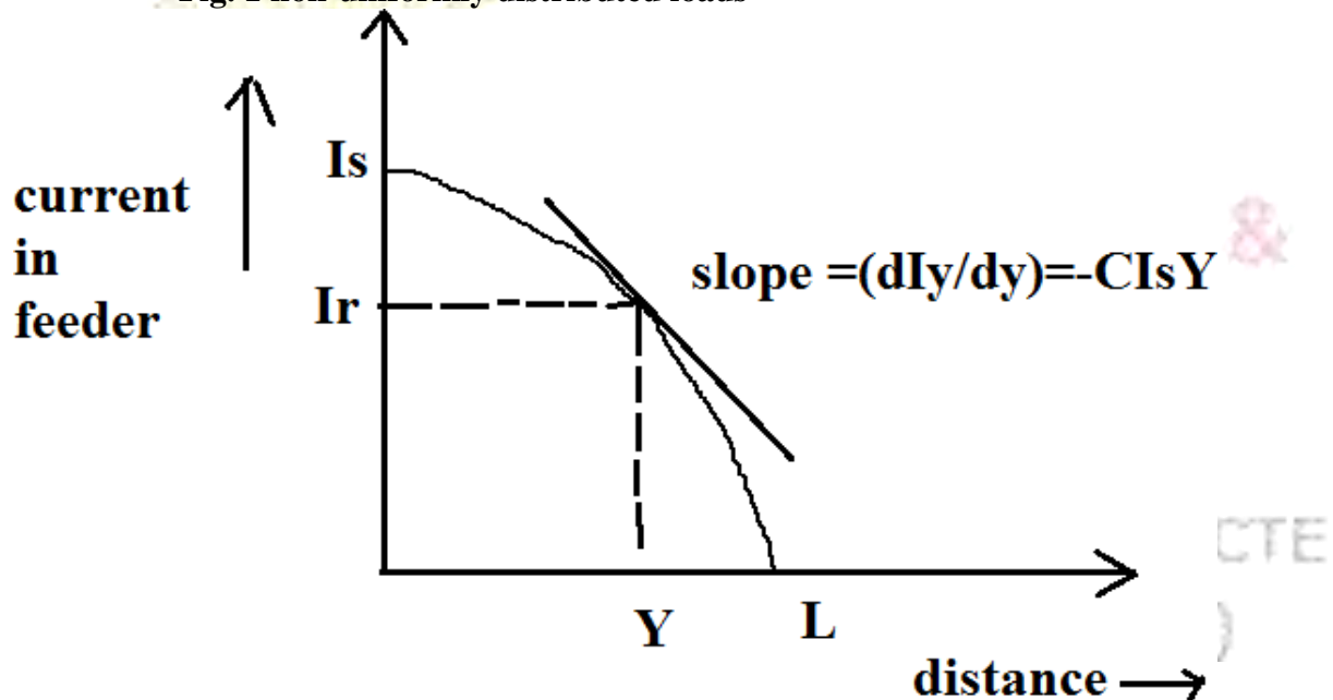
Fig. 1 non-uniformly distributed loads
