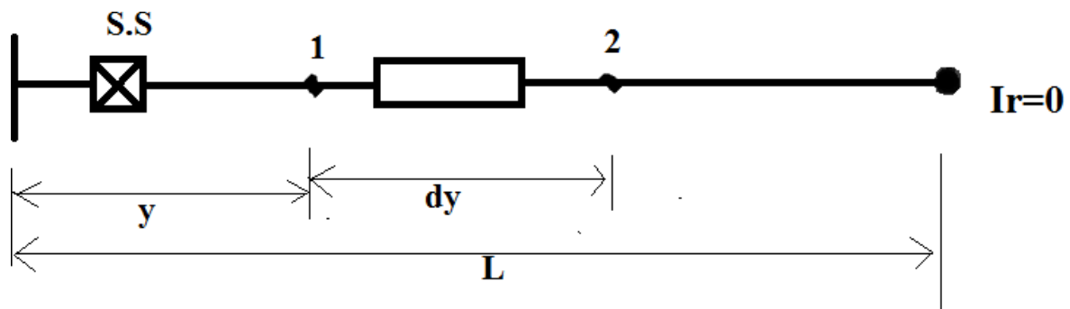
Fig:1 single line diagram of 3 phase circuit.
