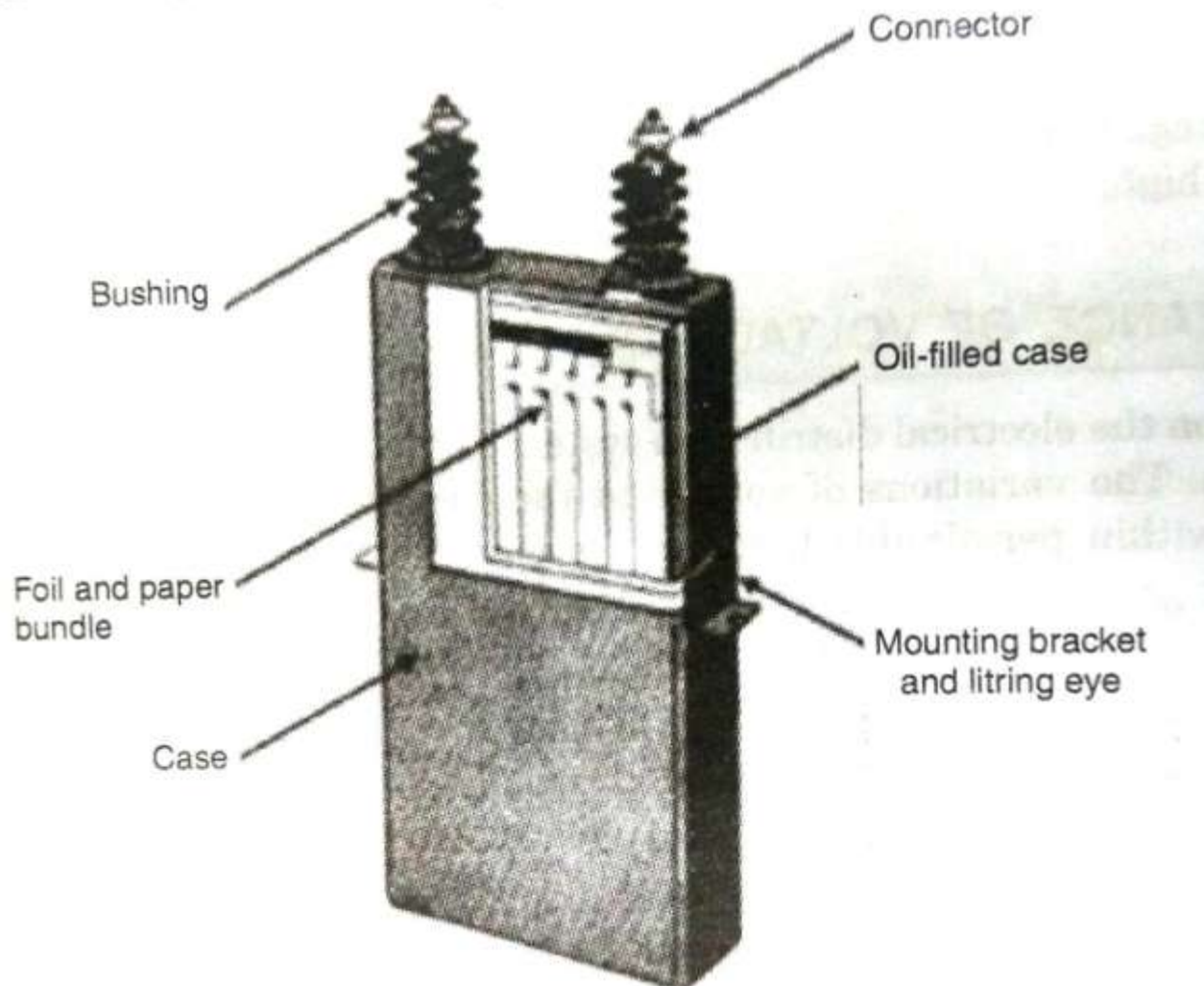
FIG 5.1 PRIMARY CAPACITOR
