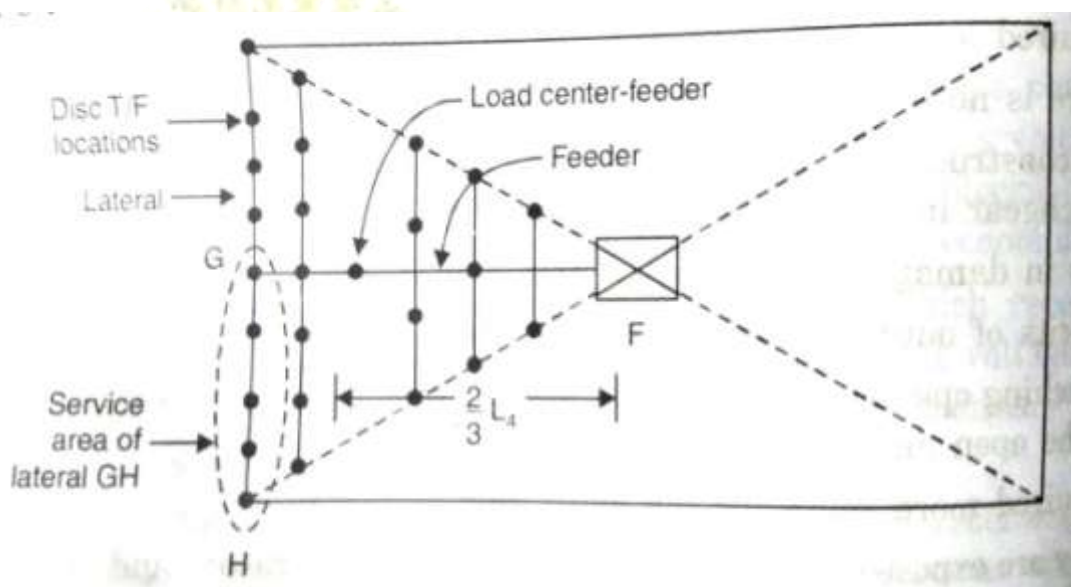
FIG SQUARE SHAPED SERVICE AREA OF DISTRIBUTION SUBSTATION
