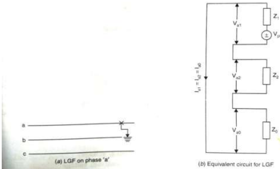
FIG SINGLE LINE TO GROUND FAULT
