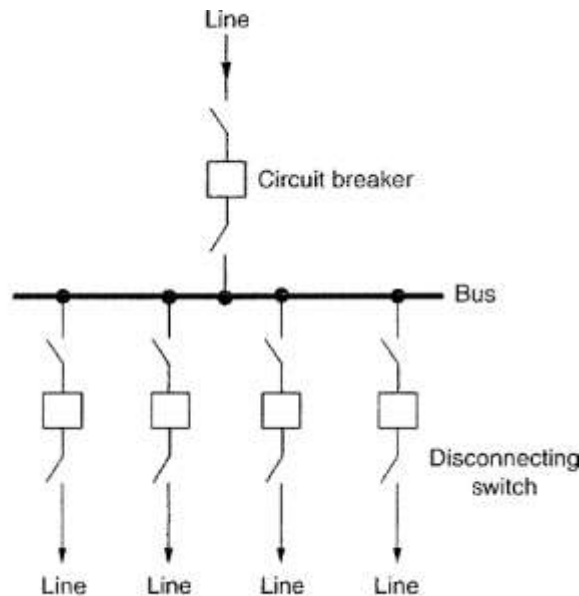
A typical single-bus scheme.
