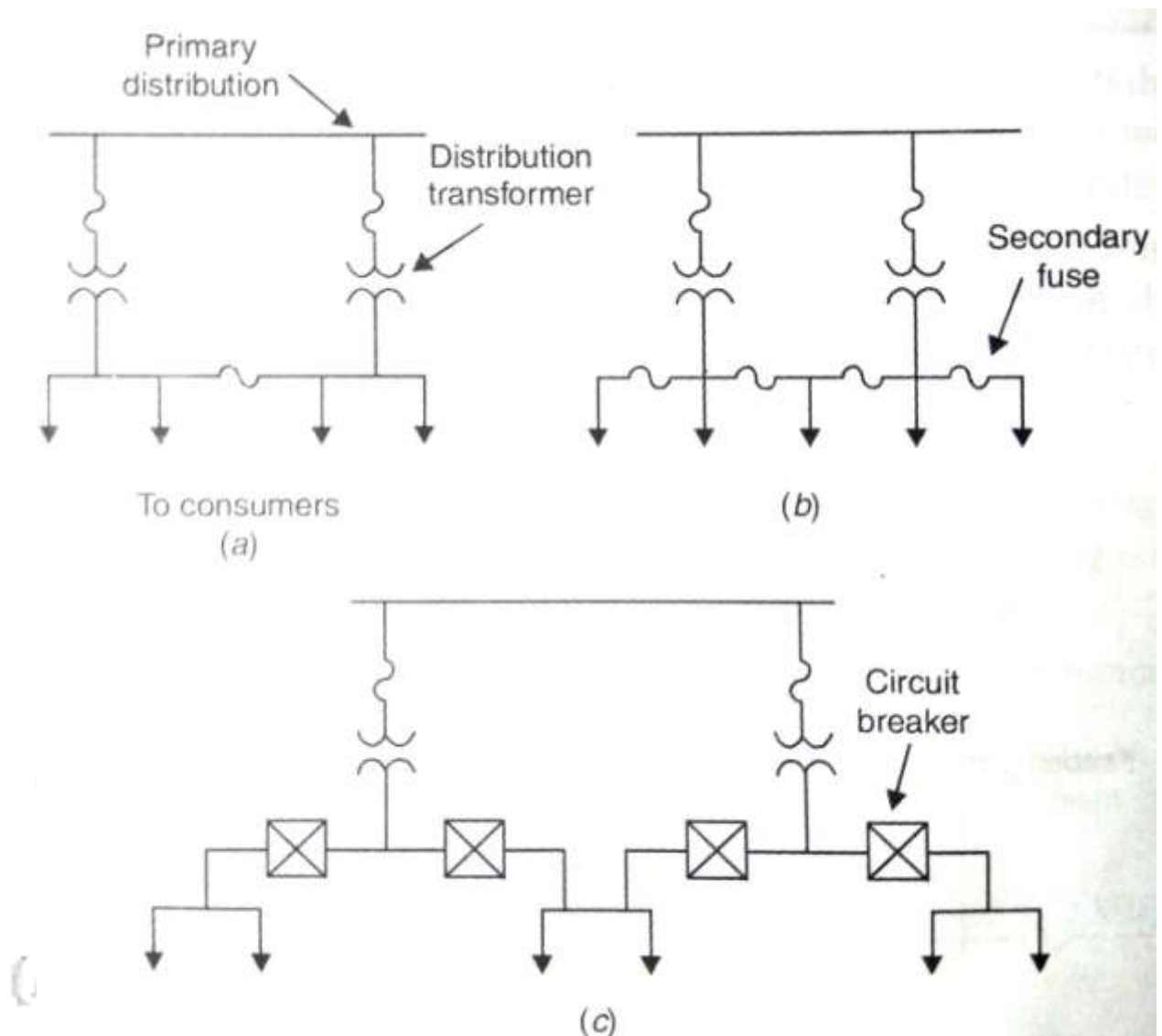
FIG 2.9 SECONDARY BANKING OF DISTRIBUTION TRANSFORMERS
