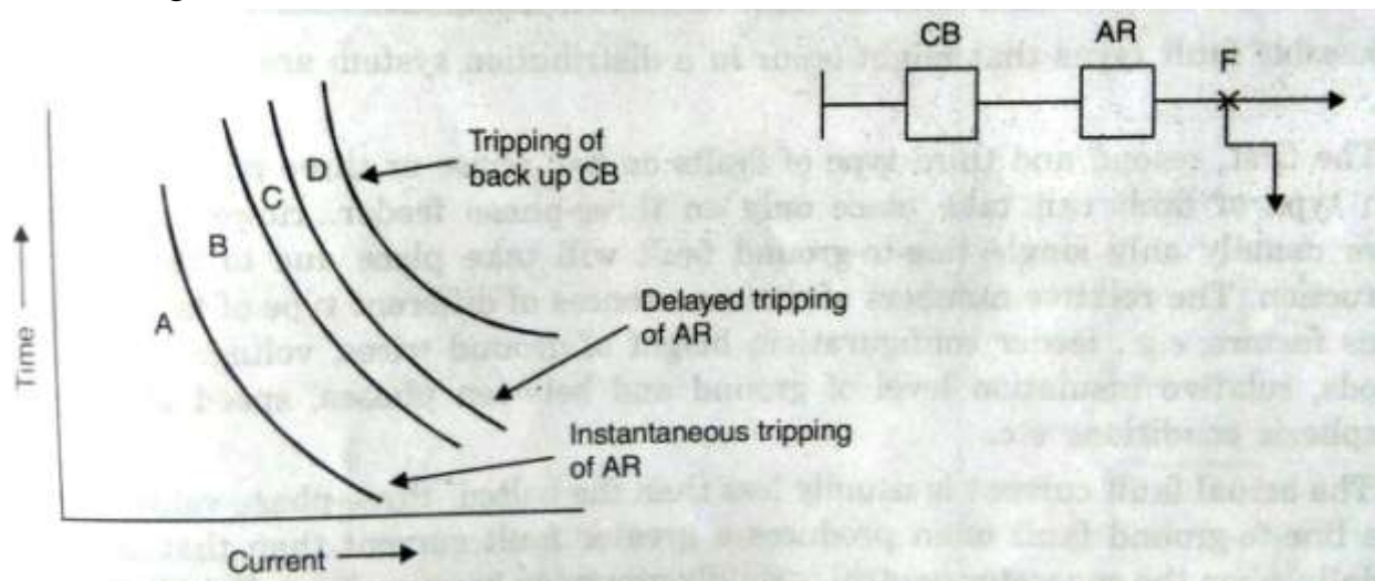
FIG CHARACTERISTICS OF CIRCUIT BREAKER TO AUTO-RECLOSER CO-ORDINATION
