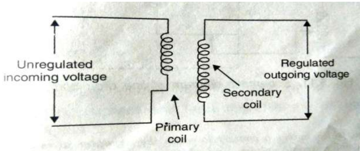
FIG 6.5 STEP TYPE VOLTAGE REGULATOR
