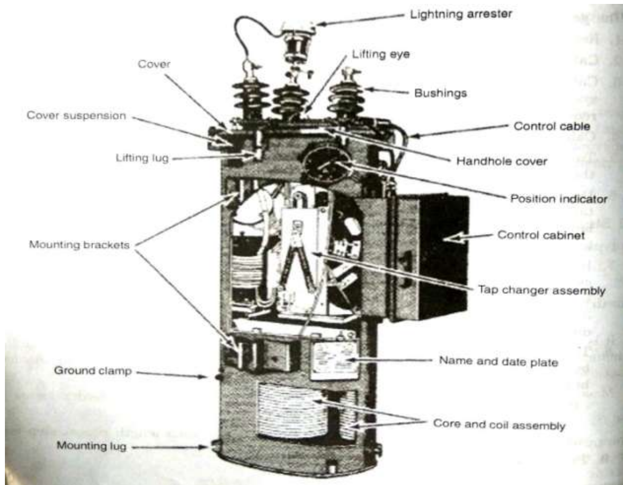
Fig 6.3 Voltage Regulator
