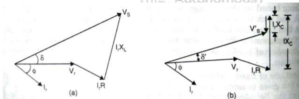
FIG 5.6 PHASOR DIAGRAM OF FIG 5.5(a) AND (B) RESPECTIVELY
