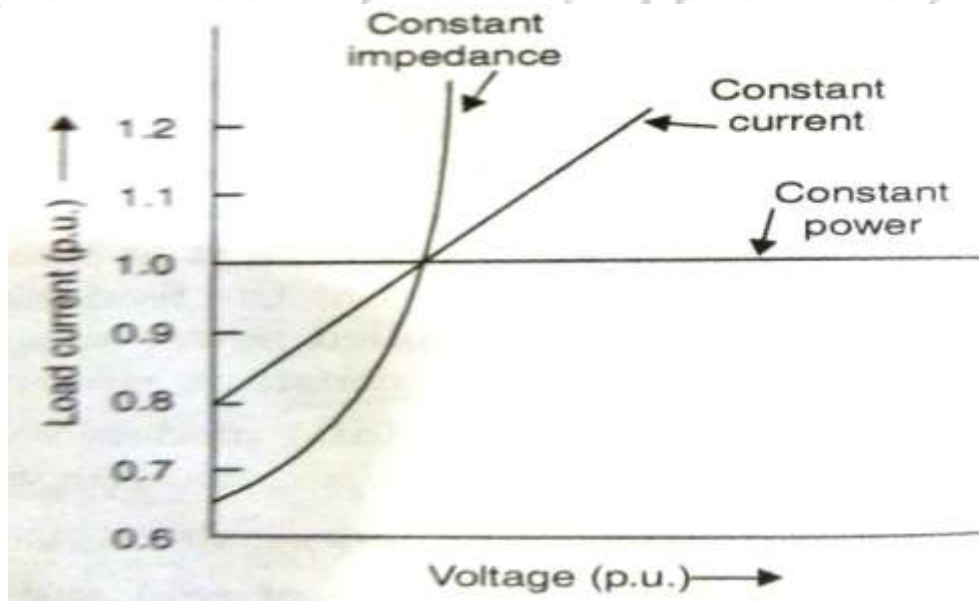
FIG RELATION BETWEEN LOAD CURRENT AND NODE VOLTAGE FOR SIMPLE LOAD TYPES
