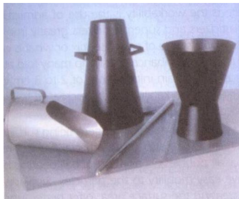
Fig 19: Slump test apparatus
