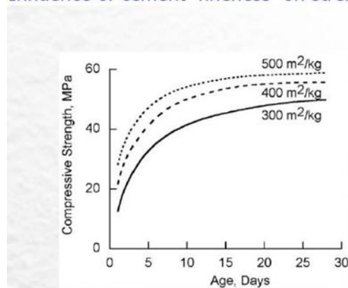
Influence of cement fineness on strength
