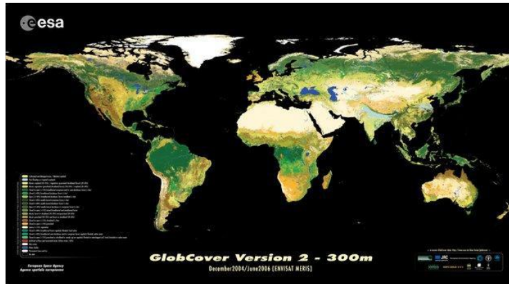
Fig. Global 300 m lands cover classification from the European Space Agency
