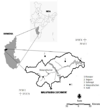
Fig. Location map of the Malaprabha catchment
