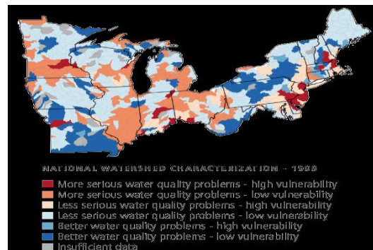
Fig. Watershed characterization of the Northern United States for water quality risk
