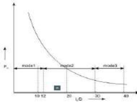
Figure 3.3 Modes of failure of columns
