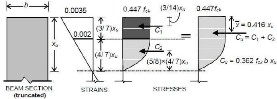
Concrete stress-block parameters in compression
