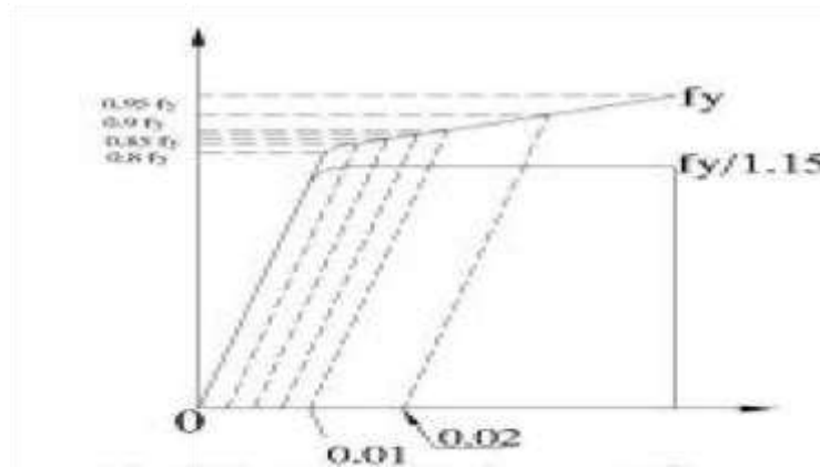
Stress-strain curve for cold worked deform bar
